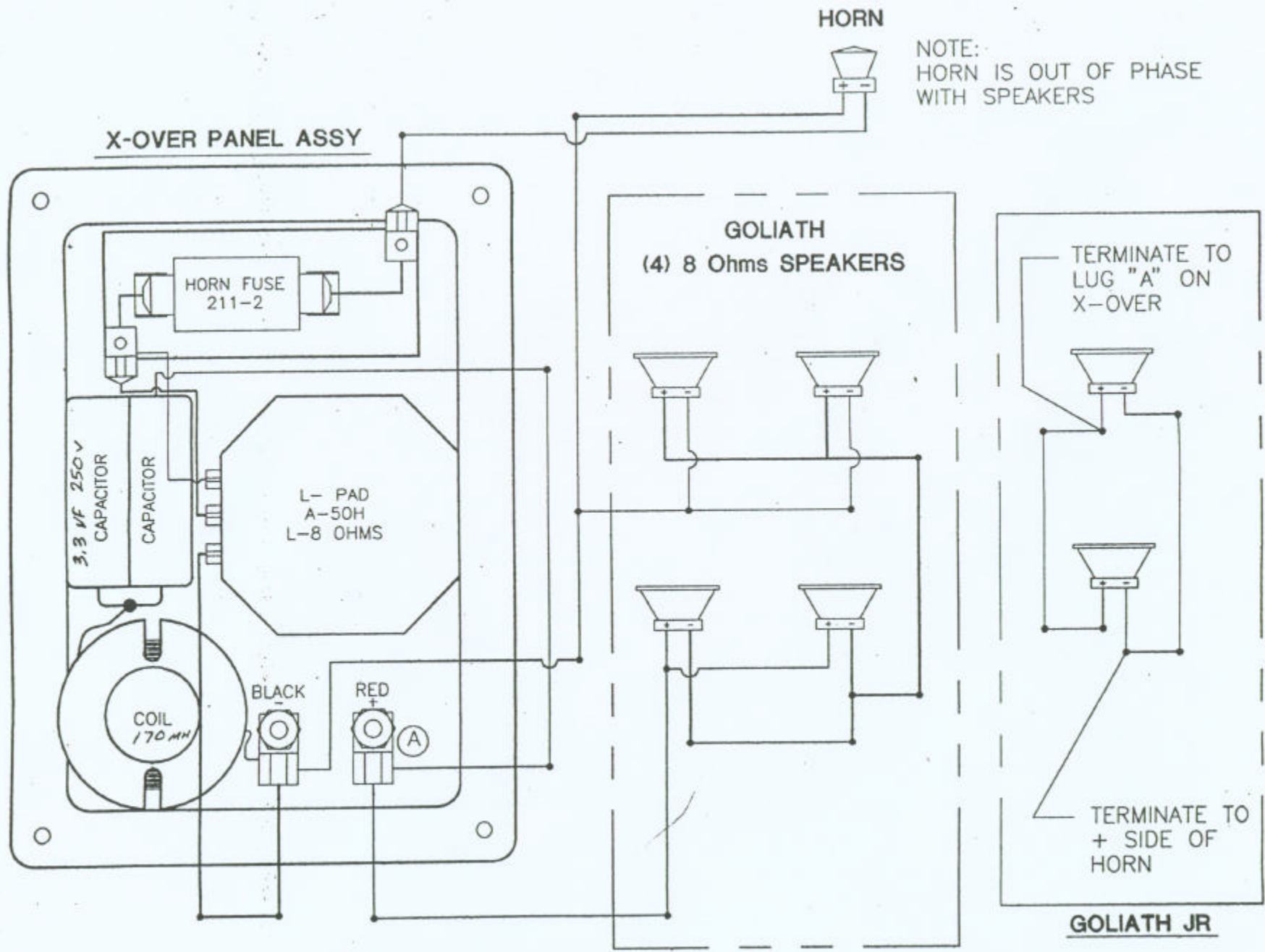
OLD STYLE X-OVER LAYOUT
